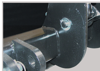
Top mast wraps around 3 sides of main beam for added strength
